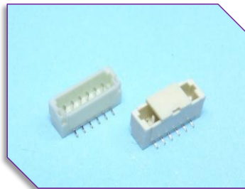
E03-W 1.00mm Wafer SMT
