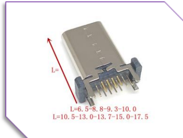
A25-F-V-A-16 USB Type C 16pin Female Vertical Dip Type
