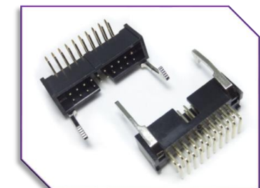
F22L 2.54mm Box Header with Metal Latch
