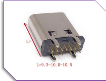
A25-F-V-A-14 USB Type C 14pin Female Vertical Dip Type
