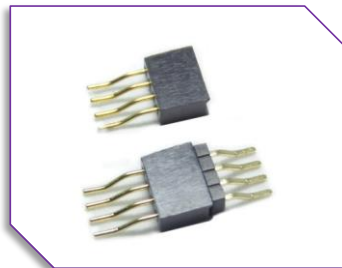
B34S 1.27mm Female Socket SMT + R/A
