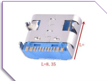
A25-F-M-J-16 USB Type C 16pin Female SMT Type
