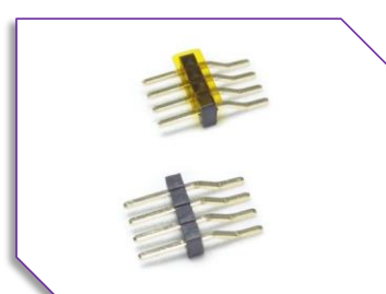
B30S 1.27mm Pin Header SMT + R/A
