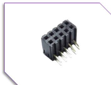
B55 1.00mm Female Socket
