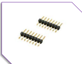
B40S 2.00mm Pin Header SMT+ R/A
