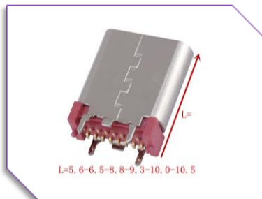
A25-F-V2-D-16 USB Type C 16pin Female Vertical SMT Type
