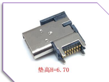
A25-F-M-B-16 USB Type C 16pin Female SMT Type
