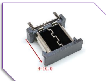
A25-F-V2-I-16 USB Type C 16pin Female Vertical SMT Type
